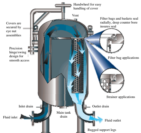
TYPICAL MULTI-FILTER
