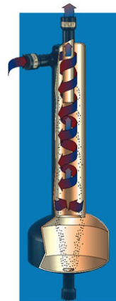
TYPICAL MULTI-FILTER
